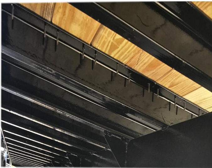
Crossmembers 12" on center
