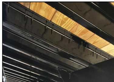
Crossmembers 12" On Center
